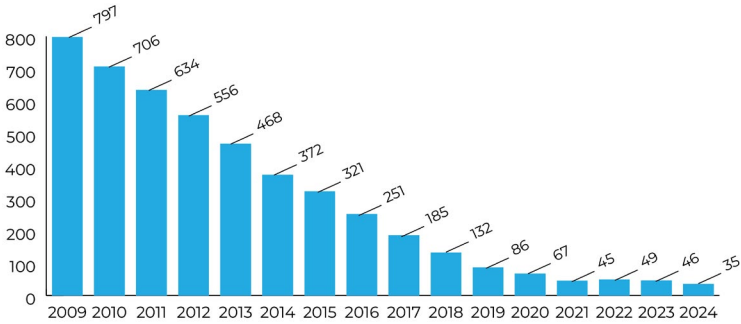
Number of Structurally Deficient Bridges
