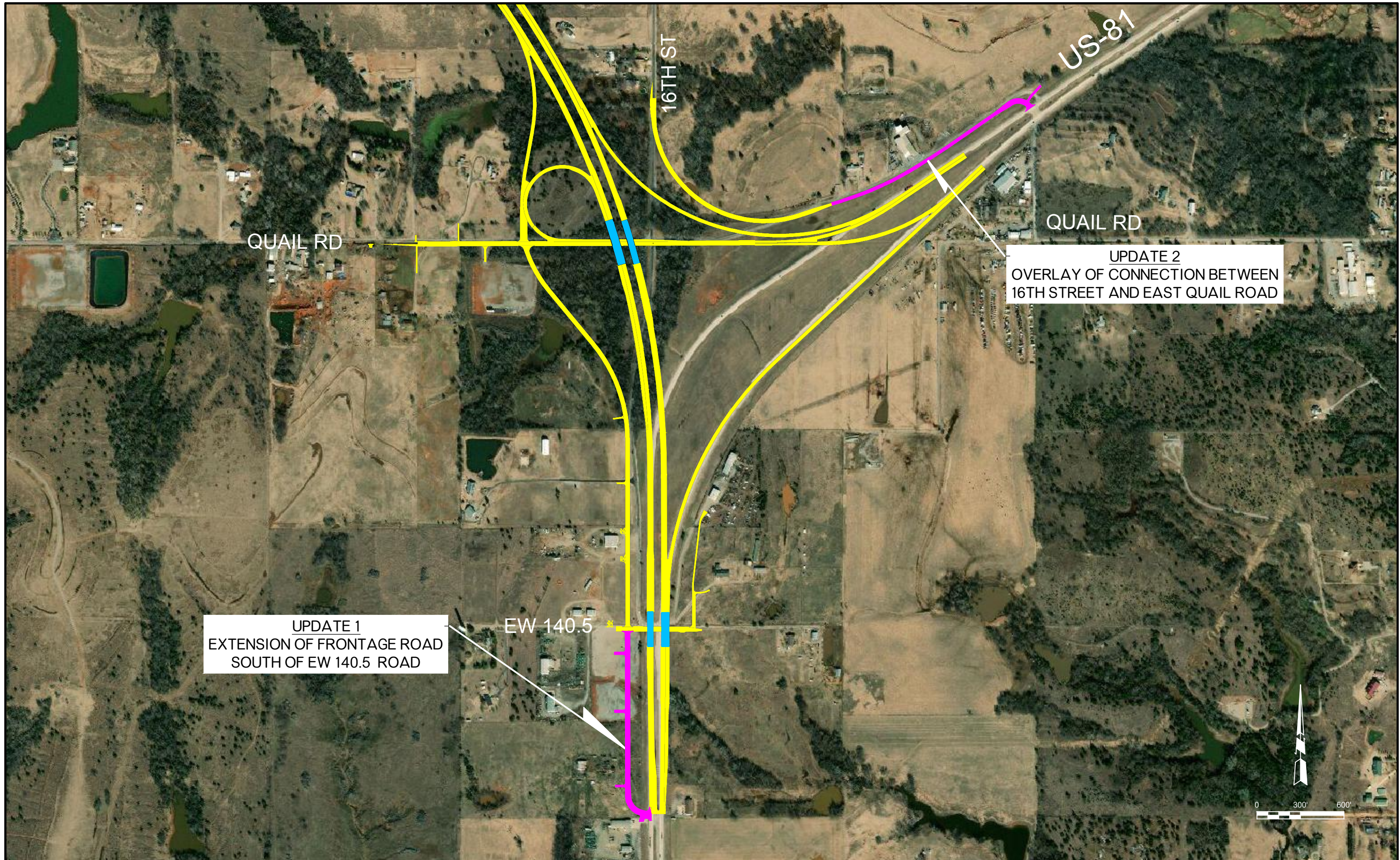
FIGURE 2 US-81 REALIGNMENT UPDATES TO ULTIMATE DESIGN
