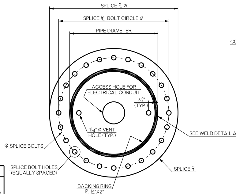
SPLICE PLATE DETAIL
