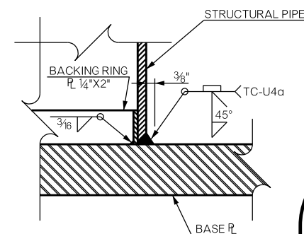
WELD DETAIL B
