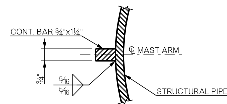
STIFFENER DETAIL
