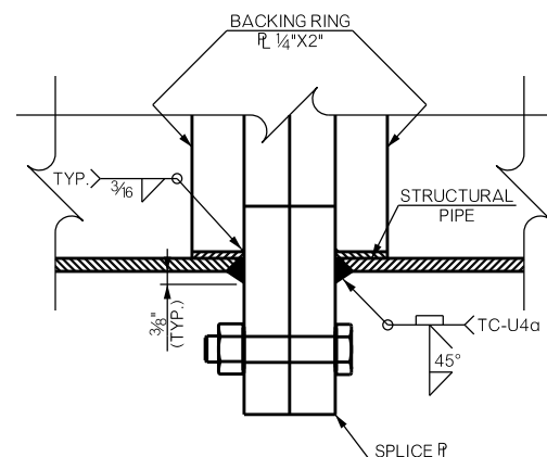
WELD DETAIL A
