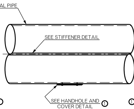
MAST ARM DETAIL
