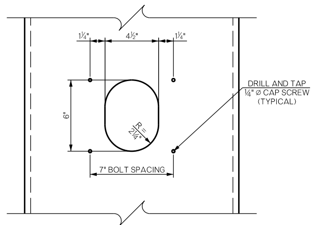
HANDHOLE AND COVER DETAIL
