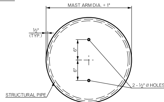
COVER PLATE DETAIL
