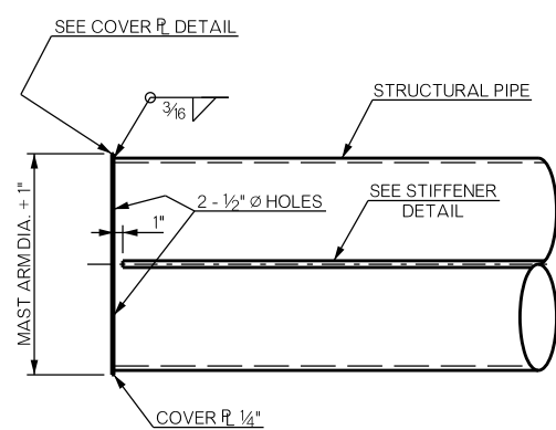
MAST ARM END DETAIL
